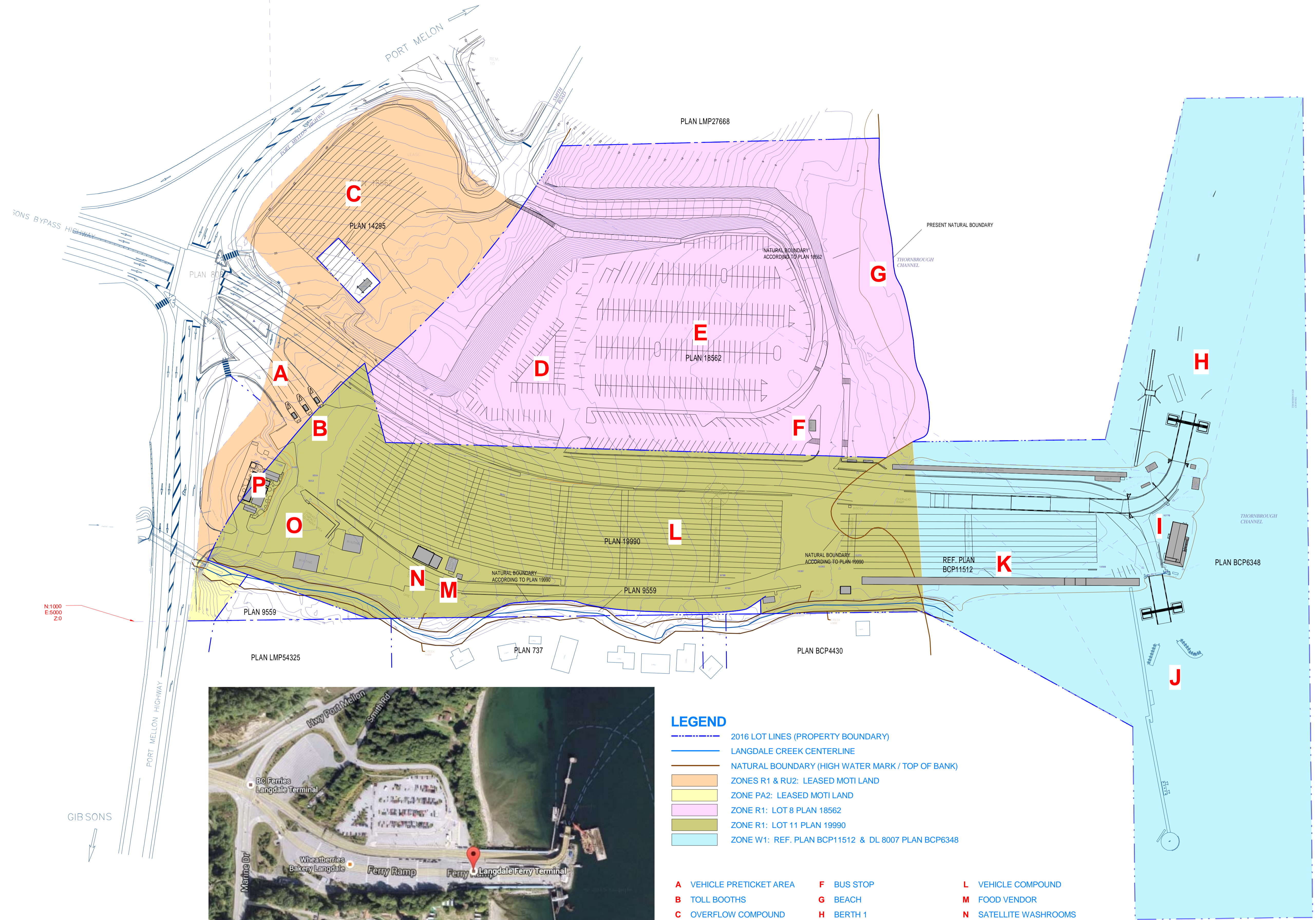
EXISTING SITE PLAN WITH 2016 ZONING NORTH 1:1000
